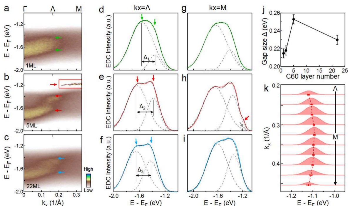
Figure 3. Thickness-dependent gap-like and sub-band features. Raw ARPES intensity maps of the HOMO band dispersion for 1 ML (a), 5 ML (b), and 22 ML (c) C_{60} films. The \Lambda point denotes the midpoint between \Gamma and M. The inset in part b shows the second-derivative image, highlighting the sub-band feature in the 5 ML film; the corresponding raw-intensity evidence is provided in Figure S3. EDCs at the \Lambda point for C_{60} films with thicknesses of 1 ML (d), 5 ML (e), and 22 ML (f), showing gap-like structures. Spectra are fitted with two Gaussian components, as shown by gray dashed curves. EDCs at the M point for C_{60} films with thicknesses of 1 ML (g), 5 ML (h), and 22 ML (i). A shoulder feature is observed in the 5 ML film and fitted with an additional Gaussian component, as indicated by arrows in part h. (j) Extracted gap size at the \Lambda point as a function of the thickness. (k) Momentum dependence of the sub-band feature in the 5 ML film along the \Lambda –M direction, showing a hole-like dispersion.
