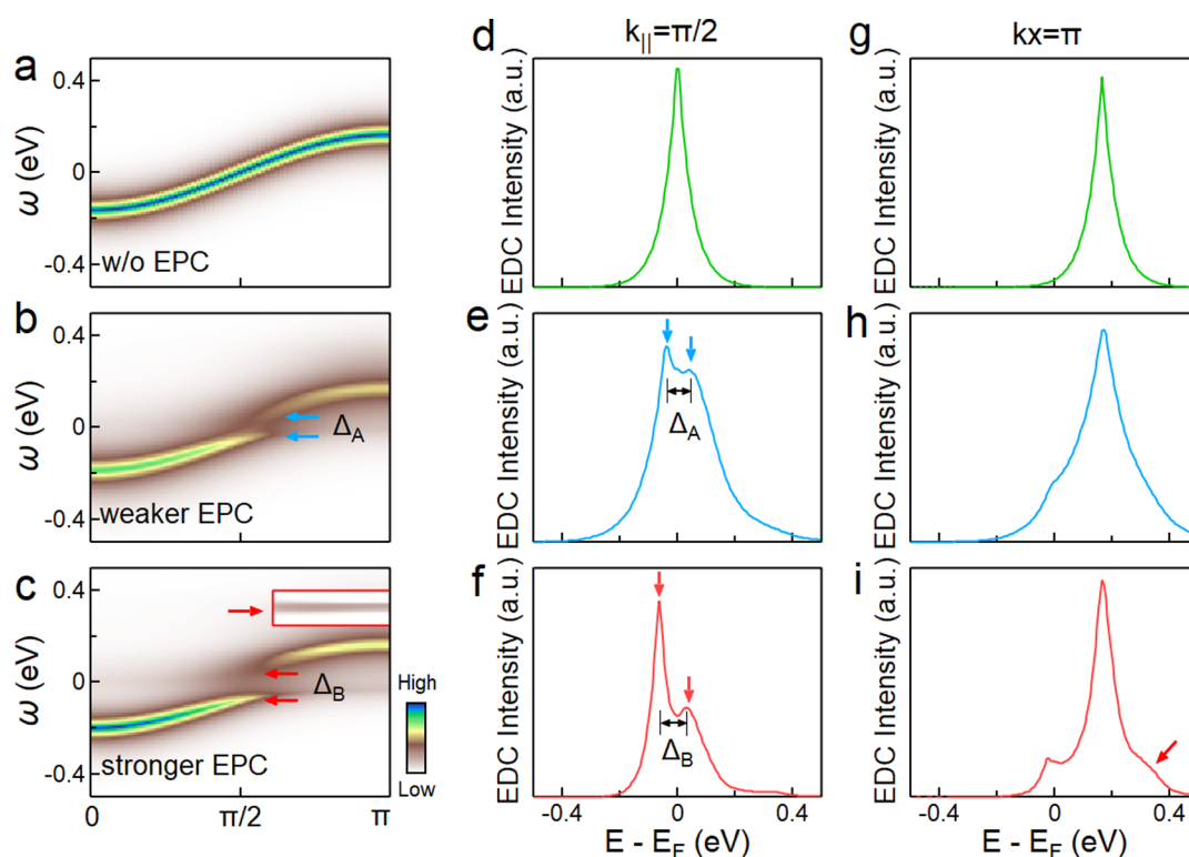
Figure 4. Simulated spectral functions with varying electron–phonon coupling strength. Simulated single-particle spectral functions of the HOMO band based on a Holstein model with coupling to the H_g(7) ( 1443\text{ cm}^{-1} ) and H_g(8) ( 1607\text{ cm}^{-1} ) intramolecular phonon modes. The mode-resolved reorganization energy ( g_m^2\omega_m ) for each of these two modes is set to 0 meV in part a, 20 meV in part b, and 30 meV in part c, corresponding to the no-coupling, intermediate-coupling, and stronger-coupling cases, respectively. Arrows indicate gap-like features and sub-band formation. (d–f) Corresponding EDCs at k_{\parallel} = \pi/2 for the three electron–phonon coupling strengths, showing the evolution from a single peak to a split structure with increasing coupling strength. (g–i) Corresponding EDCs at k_{\parallel} = \pi for the same three electron–phonon coupling strengths, showing the emergence of a sub-band feature at stronger coupling.
