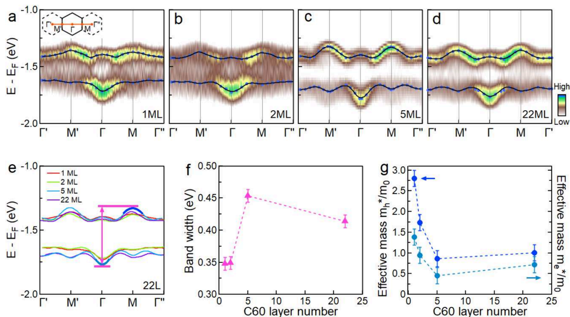
Figure 2. Thickness-dependent band dispersion and effective mass of the HOMO band. Second-derivative ARPES spectra of the HOMO band along the M'-\Gamma-M high-symmetry direction for C_{60} films with thicknesses of 1 ML (a), 2 ML (b), 5 ML (c), and 22 ML (d). Blue dots indicate extracted peak positions of the dominant HOMO-derived dispersive spectral envelope, and black curves represent fits to these features. (e) Fitted dispersions for all thicknesses overlaid for comparison. Blue curves show parabolic fits around the band top at M and the band bottom at \Gamma for the 22 ML film. The magenta arrow indicates the HOMO bandwidth ( W ) of the dominant HOMO-derived dispersive spectral envelope, defined as the energy difference between the fitted band maximum at M/M' and the fitted band minimum at \Gamma . (f) Thickness dependence of W . (g) Effective hole masses ( m_h^* ) at M/M' and electron masses ( m_e^* ) at \Gamma , extracted from local parabolic fits near the corresponding band extrema.
