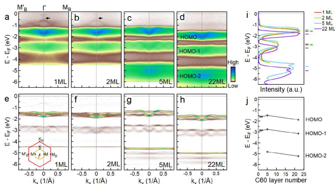
Figure 1. Thickness-dependent electronic structures of C_{60} films on a Bi_2Se_3 substrate. ARPES band structures of C_{60} films with thicknesses of 1 ML (a), 2 ML (b), 5 ML (c), and 22 ML (d), measured along the M_B'-\Gamma-M_B high-symmetry direction. Bands originating from the Bi_2Se_3 substrate are indicated by arrows in parts a and b. (e–h) Second-derivative images with respect to energy, derived from parts a–d. The Brillouin zones of C_{60} and Bi_2Se_3 are outlined in yellow and red, respectively, in the inset of part e. (i) EDCs integrated over the full M_B'-\Gamma-M_B momentum range for all four thicknesses. The colored bars on the right indicate the centroid energy of each band manifold. (j) Thickness dependence of the centroid energies of each band manifold, extracted from the EDCs.
