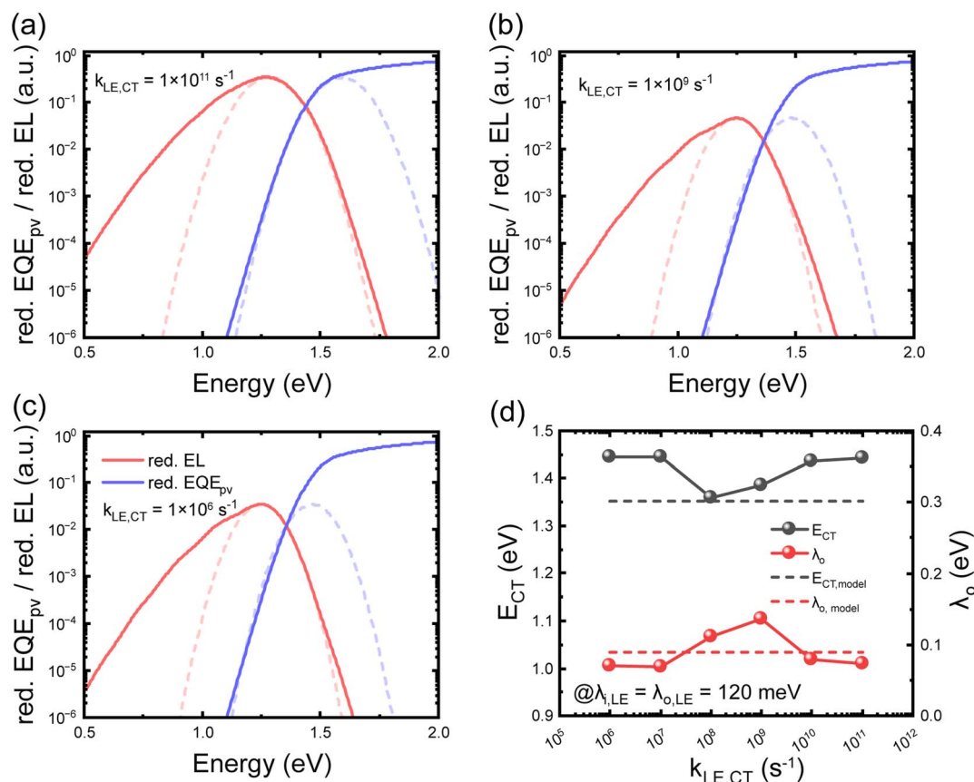
Fig. 9 Summary of the results for different rate constants of LE to CT states ( k_{LE,CT} ) with \Delta E_{LE,CT} = 0.1 \text{ eV} via fitting EL and EQE spectra using the classical Marcus theory. (a–c) Fits obtained using k_{LE,CT} values of 10^{11} , 10^9 , and 10^6 \text{ s}^{-1} , respectively. (d) Comparison between the physical parameters of the original model and the classical Marcus fit results. The previously developed model was used to generate EL and EQE data, with input parameters as shown in Note S1. The dotted line represents the parameters set in the original model, and the solid line represents the result obtained by the classical Marcus fitting. \lambda_{o,model} corresponds to the low frequency reorganization energy of the CT state in the original model, and E_{CT,model} corresponds to the free energy of the CT state.
