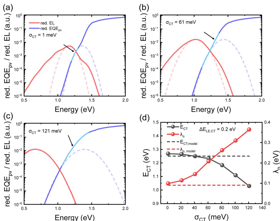
Fig. 5 Summary of the results for different static disorder ( \sigma_{\text{CT}} ) with \Delta E_{\text{LE,CT}} = 0.2 eV via fitting EL and EQE spectra using the classical Marcus theory. When performing Marcus fitting on the results with static disorder of (a) 1 meV, (b) 61 meV, and (c) 121 meV, the bright blue curve segment is a reference marker indicating the downward shift of the main peak of the red. EL spectrum. (d) Comparison between the physical parameters of the original model and the classical Marcus fit results. The previously developed model was used to generate EL and EQE data, with input parameters as shown in Note S1. The dotted line represents the parameters set in the original model, and the solid line represents the result obtained by the classical Marcus fitting. \lambda_{o,\text{model}} corresponds to the low frequency reorganization energy of the CT state in the original model, and E_{\text{CT,model}} corresponds to the free energy of the CT state.
